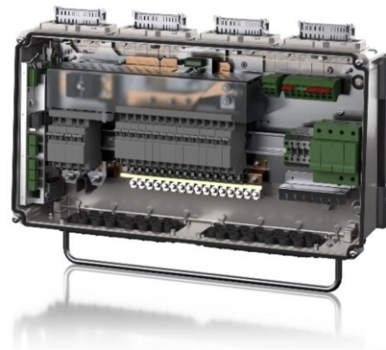
System Compartment Interior
